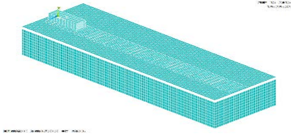
Fig. 2: Three-dimensional finite element model of ballasted railway track
