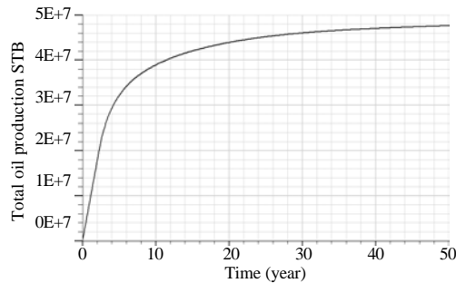
Fig. 3: Cumulative production during natural depletion mechanism without drilling new production wells and EOR operation
