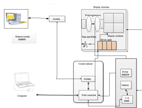
Fig. 1: Display system
