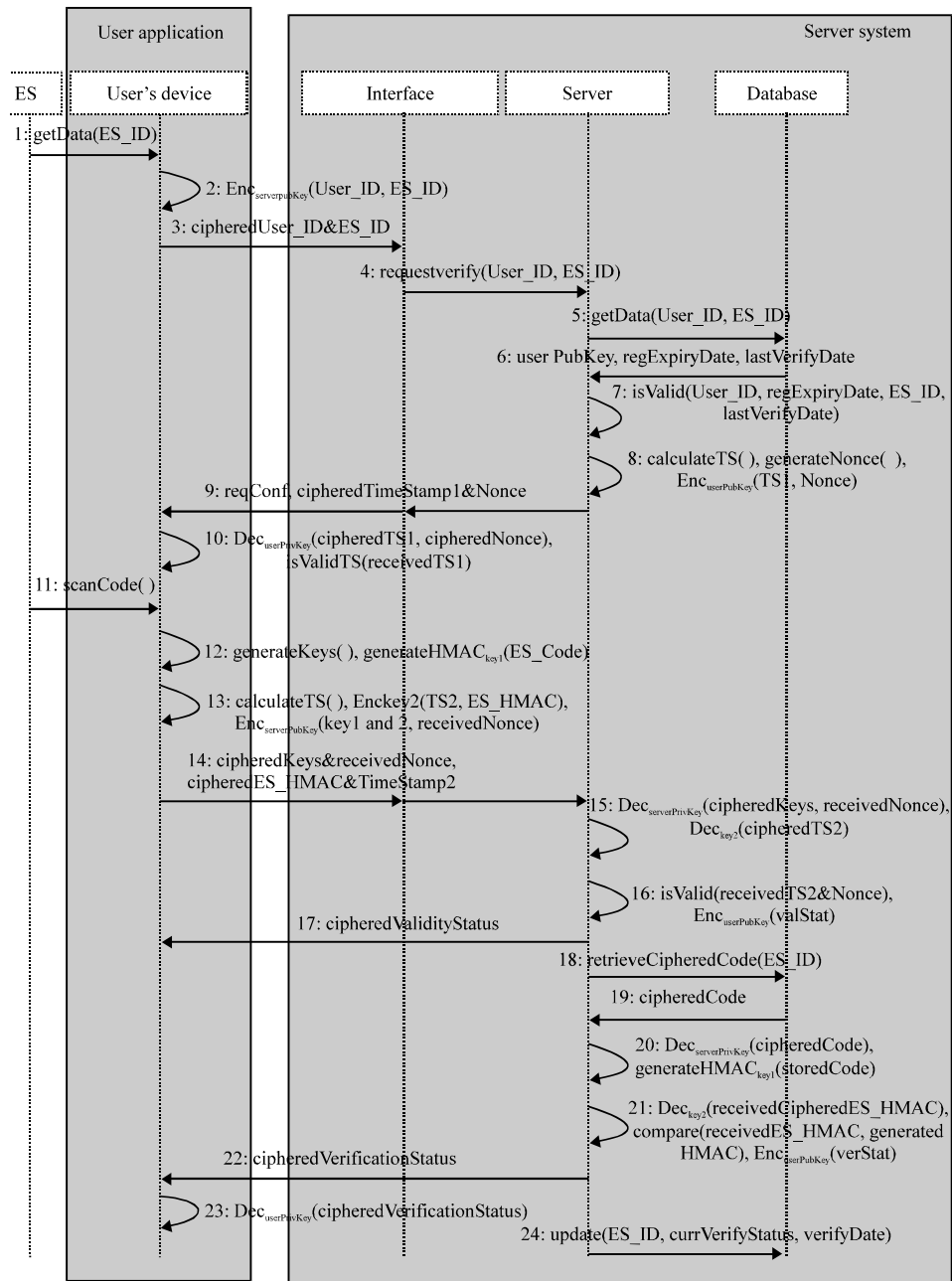
Fig. 2: Remote code integrity verification protocol
